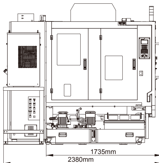
Left View
